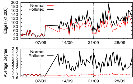
Figure 7: The changes in average degree (bottom) and the number of edges (top) of the Web TDG after we inject Gnutella traffic. Plots show both the values of the metrics under no pollution (normal) and after pollution (polluted).
