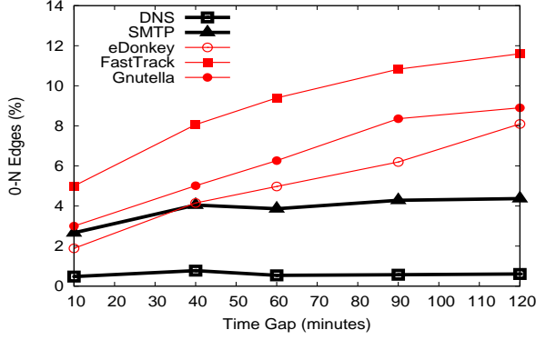
Figure 2: The “edge volatility” of five different applications over time. All P2P TDGs change more over time compared to the SMTP and DNS TDGs.
