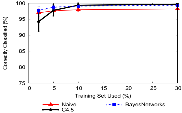
Figure 3: Collaborative vs Non-Collaborative applications: graph classification performance using static metrics. For each experiment we executed 50 runs with different random training samples.
