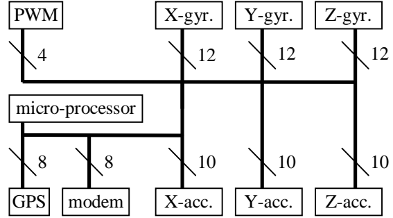
Figure 2. Bus structure for GPS Navigation System.
