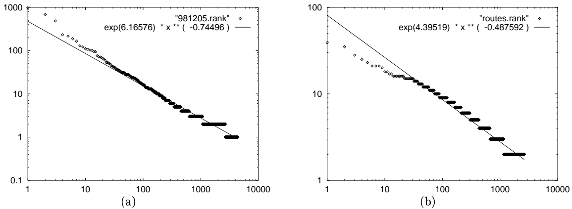
Figure 4: The rank plots. Log-log plot of the outdegree d_v versus the rank r_v in the sequence of decreasing outdegree: (a) Int-12-98 (b) Rout-95.
