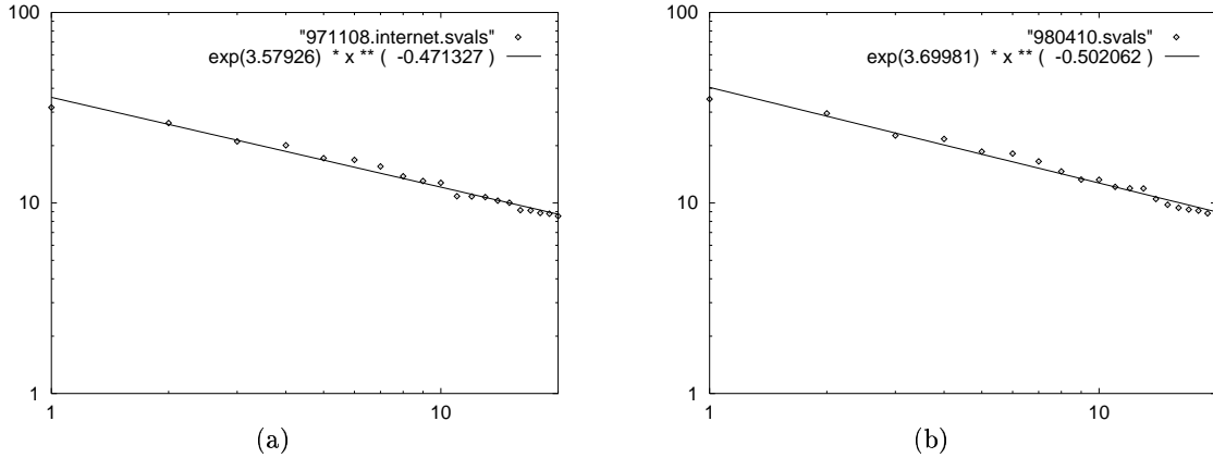
Figure 10: The eigenvalue plots: Log-log plot of eigenvalues in decreasing order (a) Int-11-97 (b) Int-04-98
