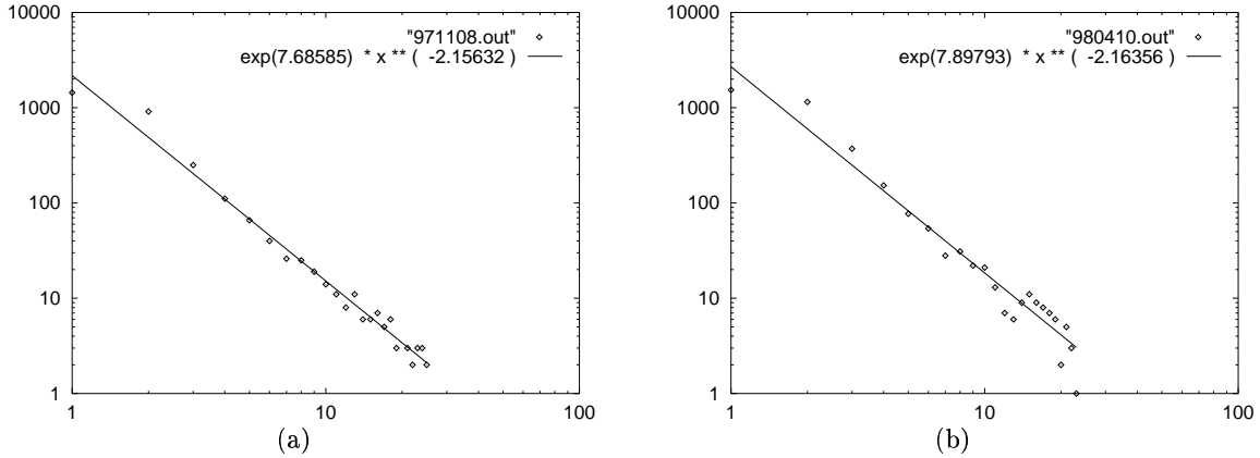
Figure 5: The outdegree plots: Log-log plot of frequency f_d versus the outdegree d : (a) Int-11-97 (b) Int-04-98.
