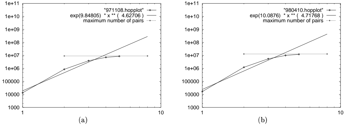
Figure 7: The hop-plots: Log-log plots of the number of pairs of nodes P(h) within h hops versus the number of hops h for (a) Int-11-97 (b) Int-04-98.
