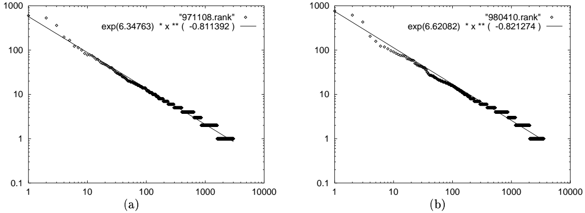
Figure 3: The rank plots. Log-log plot of the outdegree d_v versus the rank r_v in the sequence of decreasing outdegree: (a) Int-11-97 (b) Int-04-98
