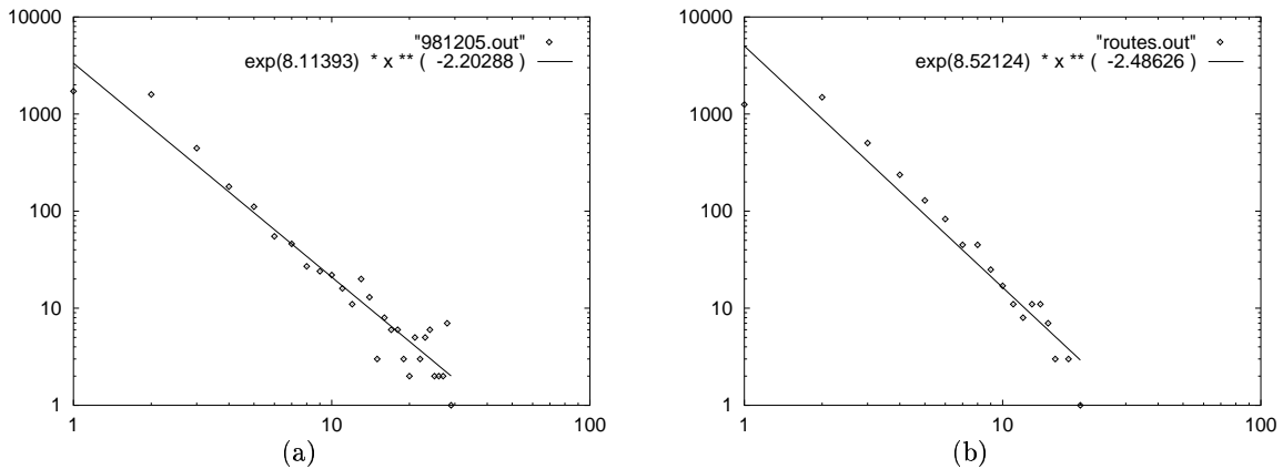
Figure 6: The outdegree plots: Log-log plot of frequency f_d versus the outdegree d : (a) Int-12-98 (b) Rout-95.
