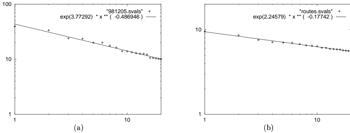
Figure 11: The eigenvalue plots: Log-log plot of eigenvalues in decreasing order (a) Int-12-98 (b) Rout-95
