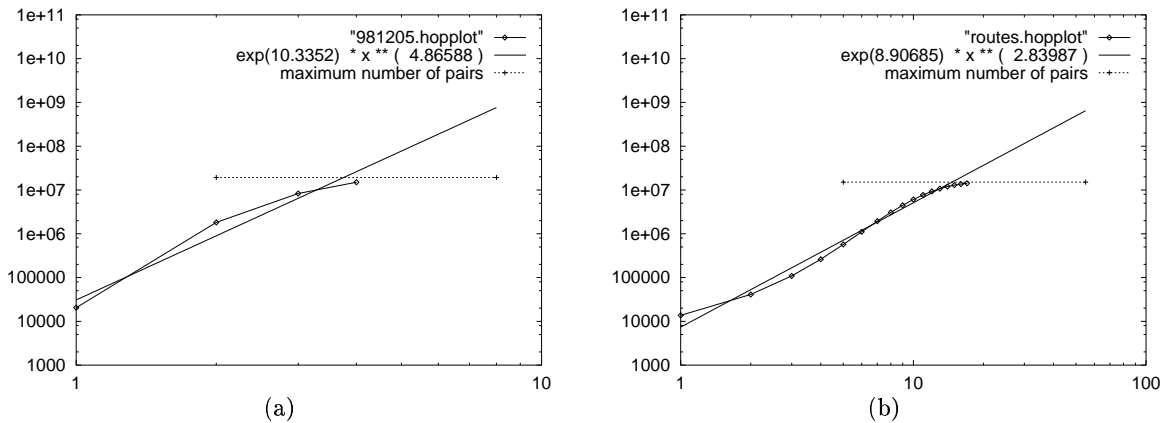
Figure 8: The hop-plots: Log-log plots of the number of pairs of nodes P(h) within h hops versus the number of hops h for (a) Int-12-98 (b) Rout-95.
